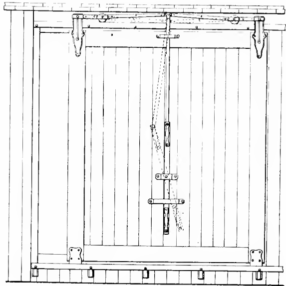
Fig. 1865. Side Elevation.
